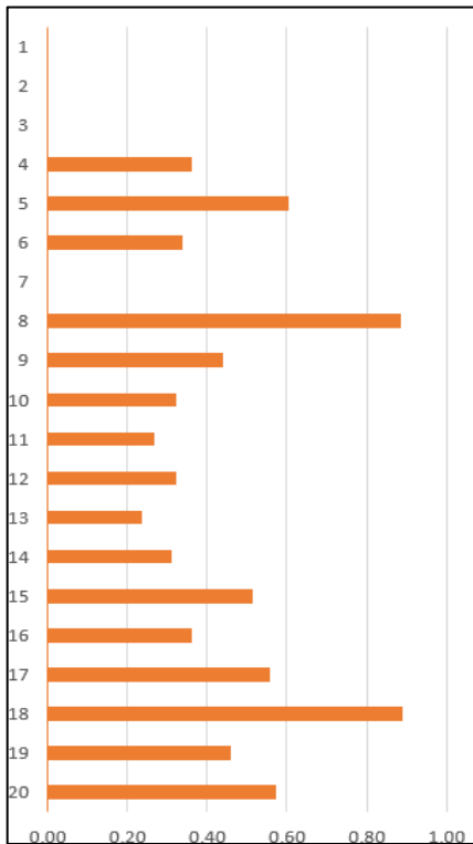
Fig. 4. Reservoir heterogeneity ranking based on image log heterogeneity index in well 2.
