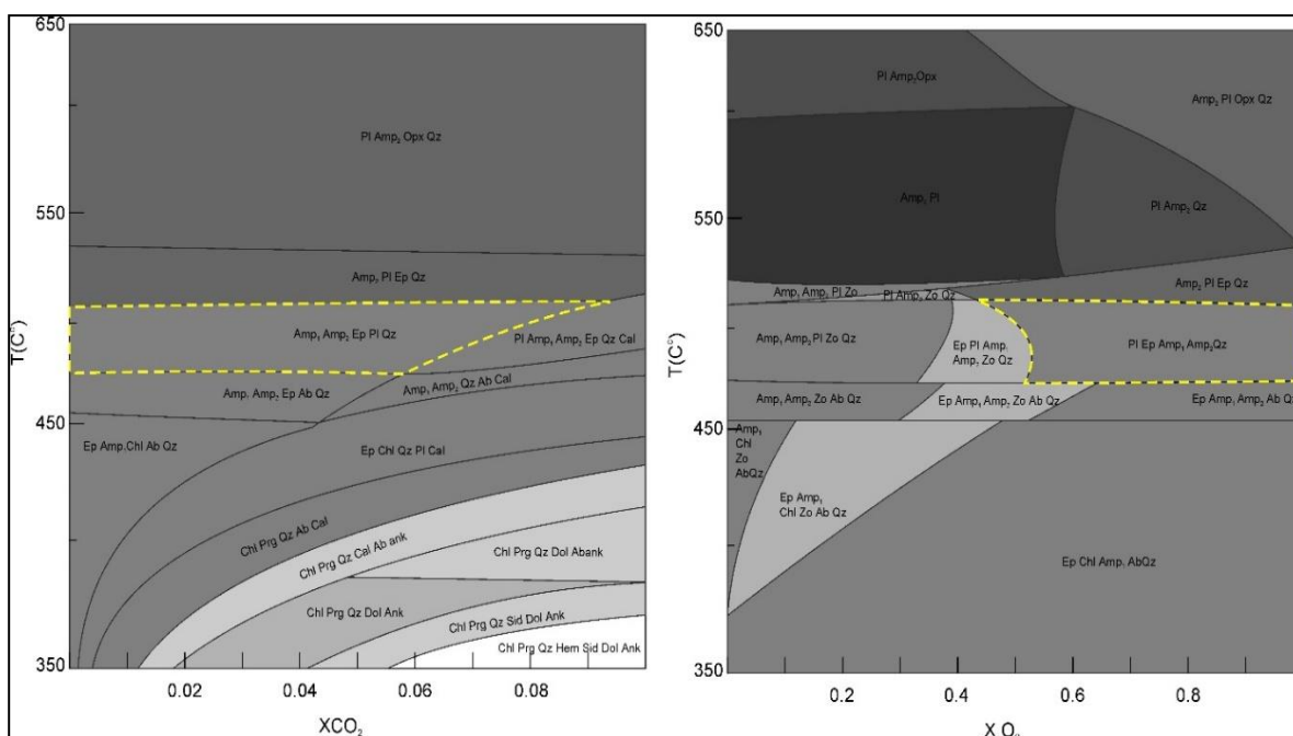
Fig. 9. (a) T-XCO_2 and (b) T-XO_2 phase diagrams calculated using EA01 sample composition. The mineral abbreviations are as Fig. 7. The dash-lines show boundaries between the stable assemblages in the studied samples and the other assemblages.
